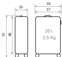
Trolley 55cm - Ref. 64811-22
